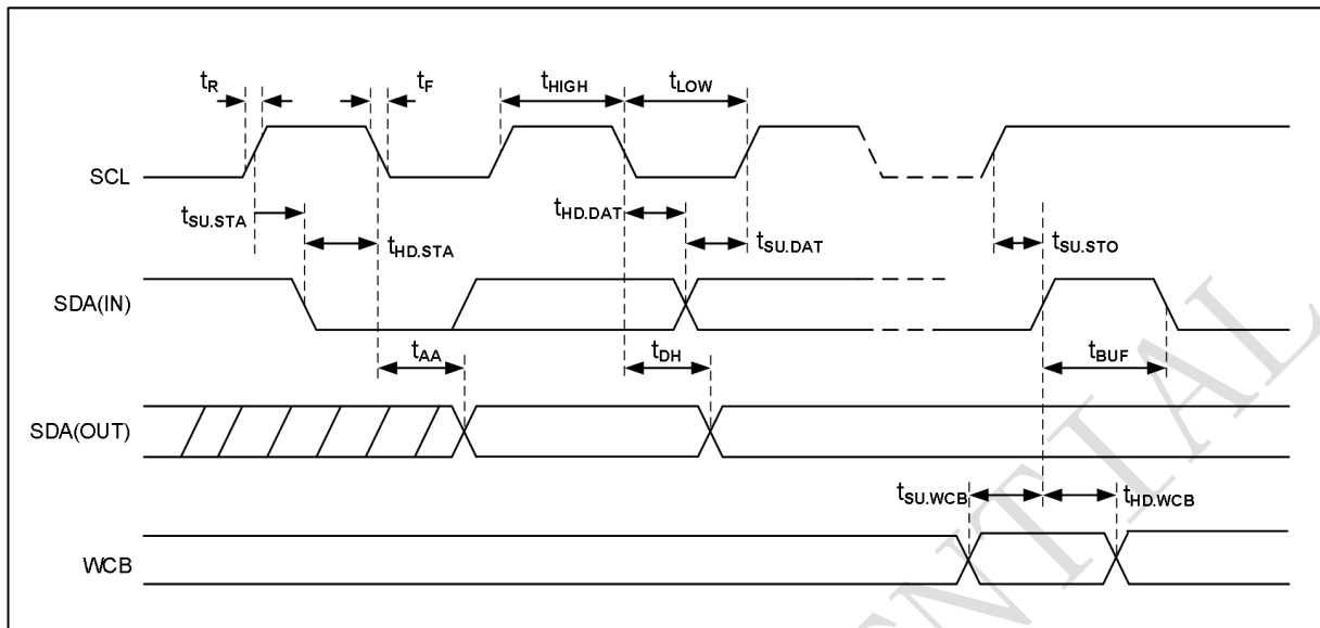
Figure 3-1 Bus Timing
